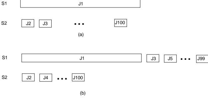
Figure 5. Server queues under (a) JSQ, and (b) LC.
