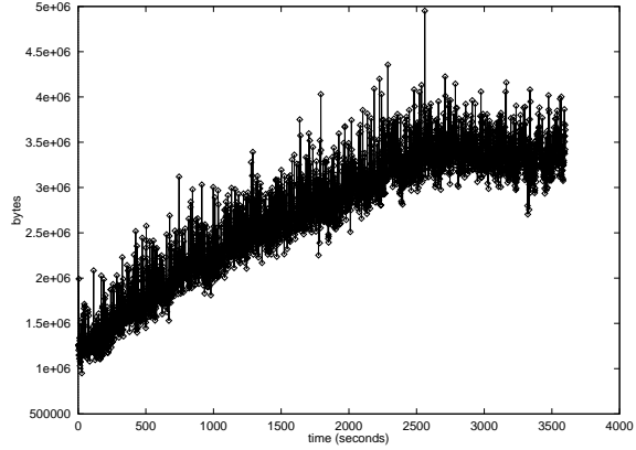
(b) Total bytes requested per second
