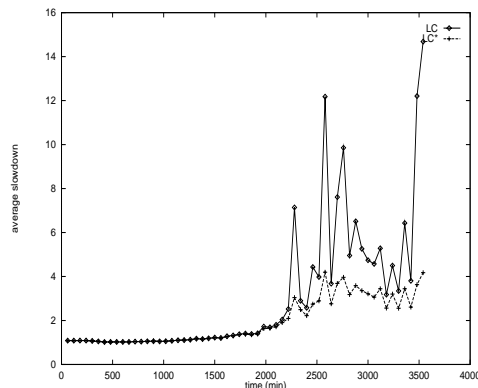
Figure 6. Successive average slowdowns for LC and LC*.
