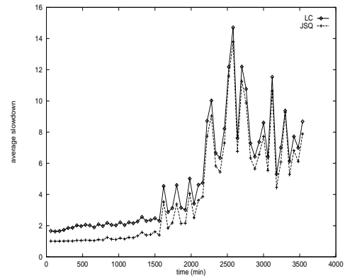
Figure 3. Successive average slowdowns of LC and JSQ when jobs are processed without preemption.
