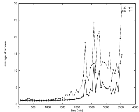
Figure 4. Successive average slowdowns of LC and JSQ when jobs are processed with preemption.
